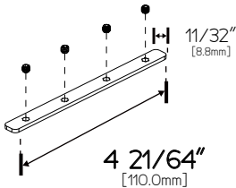
CN2001 Connector
